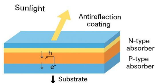
Figure 1: Structure and working principle of thin-film photovoltaic
